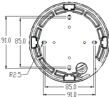
Figure 7.1 Bottom view
